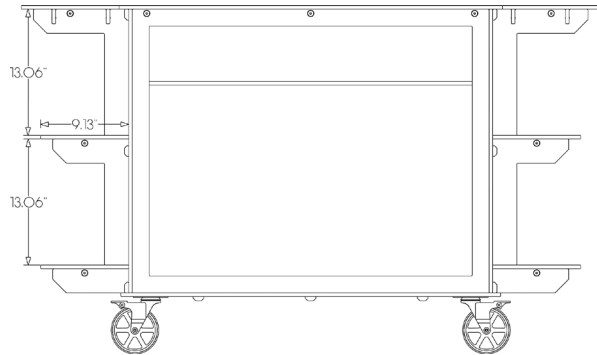
SIDE SHELVES
