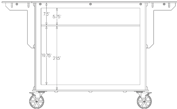
INTERIOR SHELF
